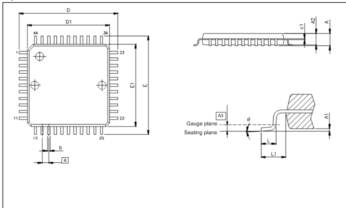
LQFP44
